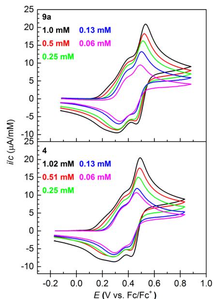
Figure 5. Cyclic voltammograms of 9a (top) and 4 (bottom) in CH 2 Cl 2 + 0.1 M Bu 4 NPF 6 recorded at a glassy-carbon working electrode at different concentrations.
